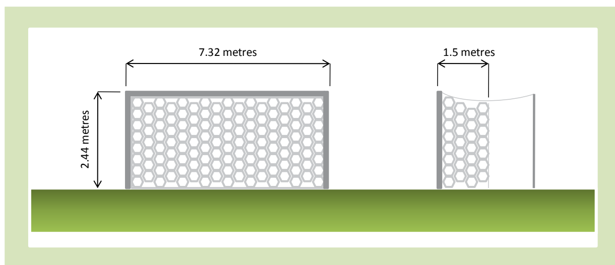
Diagram 5 - Goalpost Dimensions
